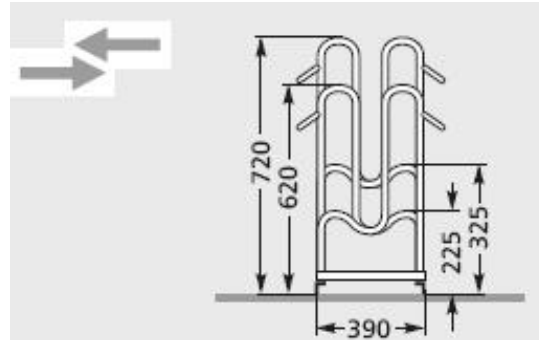
optional Bodenmontage-Winkel Art. 105000002
